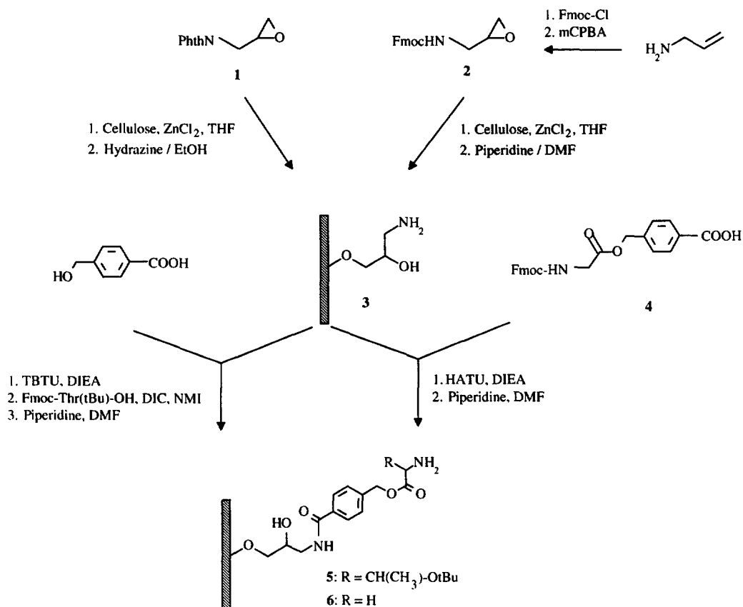
Figure 1: Synthetic scheme for the attachment of the HMB linker to the cellulose membrane
