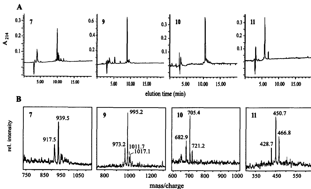
Figure 2: RP-HPLC profiles (A) and MALDI-TOF mass spectra (B) of the crude products (7, 9-11) synthesized on 5 or 6. HPLC: linear gradient 5%-40% acetonitrile/water (0.05% TFA) for 20 min at 1.2 ml/min flow rate on a RP-C 18 column. MALDI-TOF: matrix: \alpha -cyano-cinamic-acid (see also Tab. 1).
